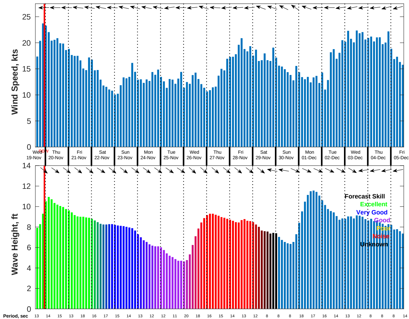
Wind & Wave Forecast for NDBC 51000 from 19-Nov-2025 14:00:00 to 05-Dec-2025 14:00:00
