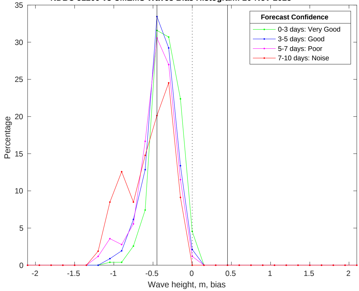
NDBC 51209 vs CMEMS Waves Bias Histogram: 20-Nov-2025
