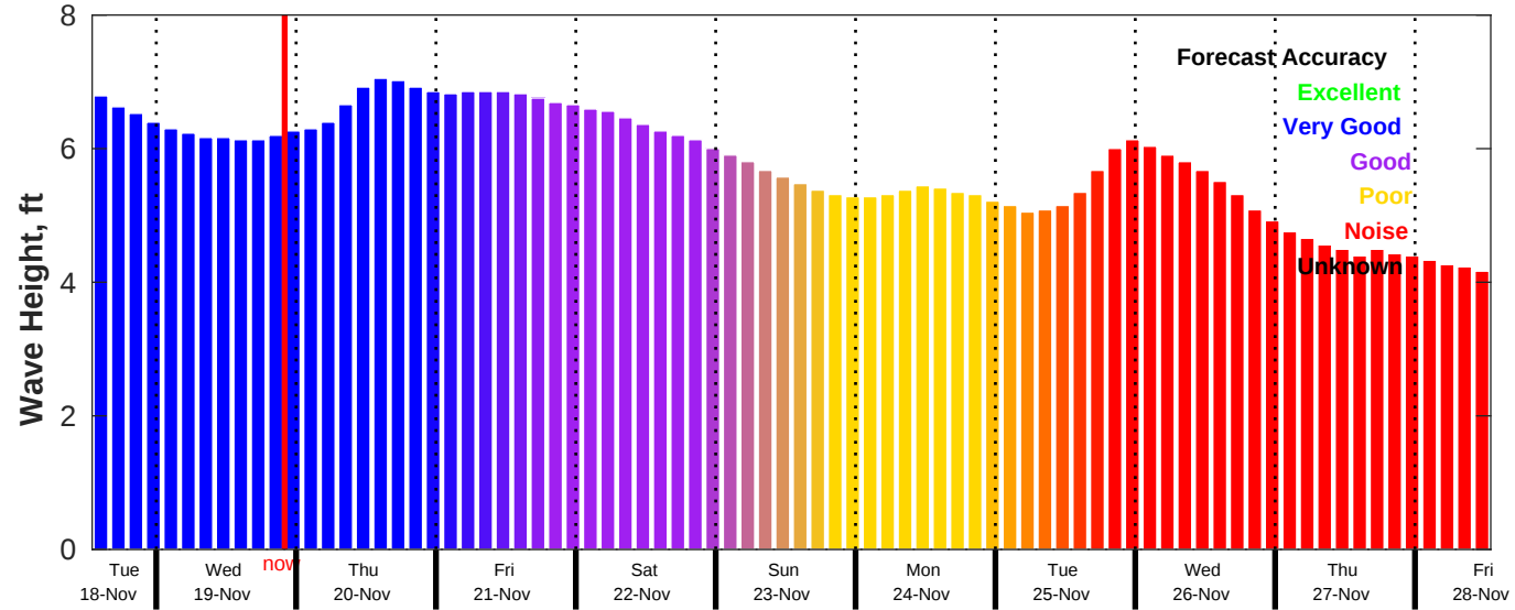
CMEMS Wave Forecast for NDBC 51209 from 18-Nov-2025 13:00:00 to 28-Nov-2025 13:00:00
