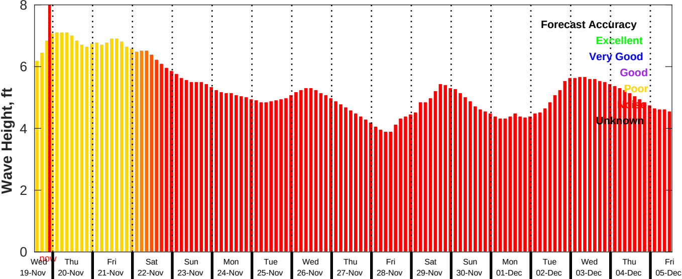
GFS Wave Forecast for NDBC 51209 from 19-Nov-2025 13:00:00 to 05-Dec-2025 13:00:00
