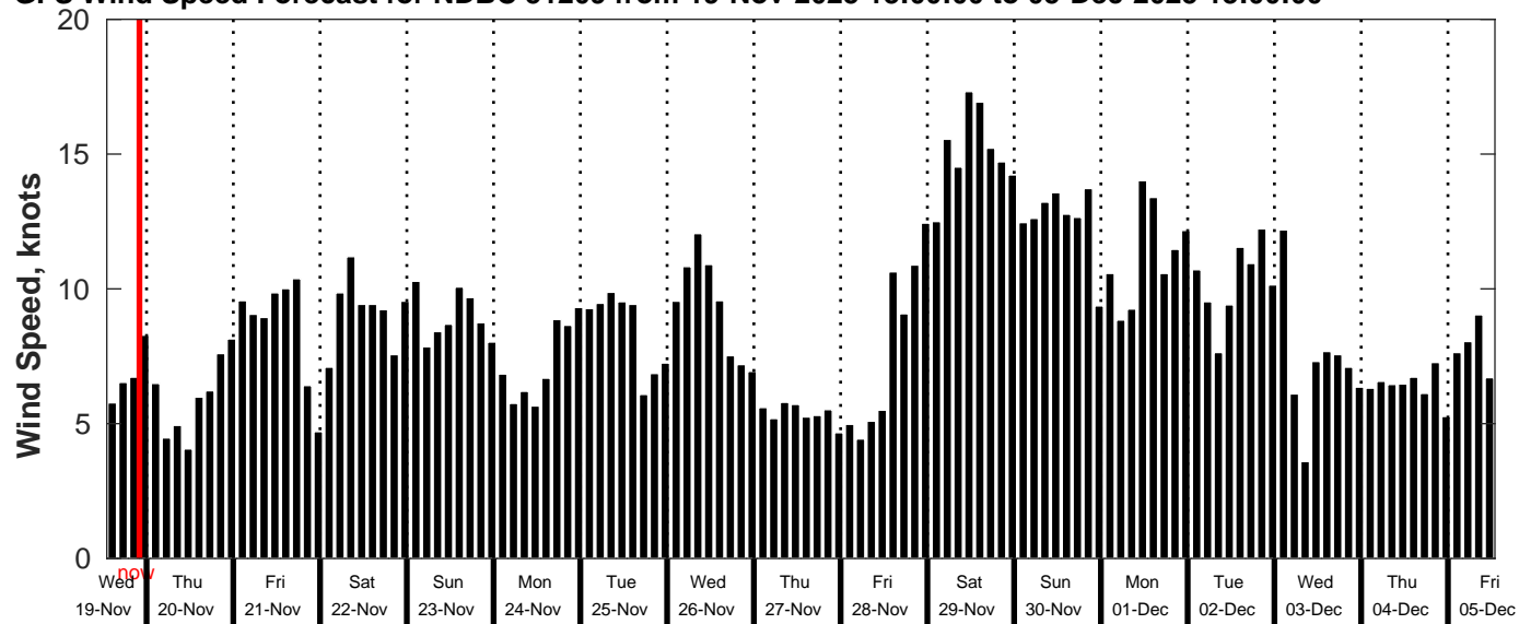
GFS Wind Speed Forecast for NDBC 51209 from 19-Nov-2025 13:00:00 to 05-Dec-2025 13:00:00
