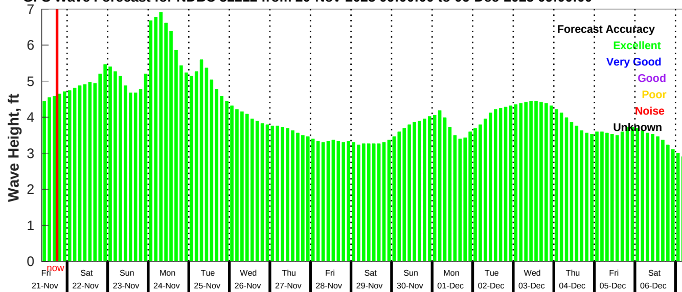
GFS Wave Forecast for NDBC 52212 from 20-Nov-2025 09:00:00 to 06-Dec-2025 09:00:00
