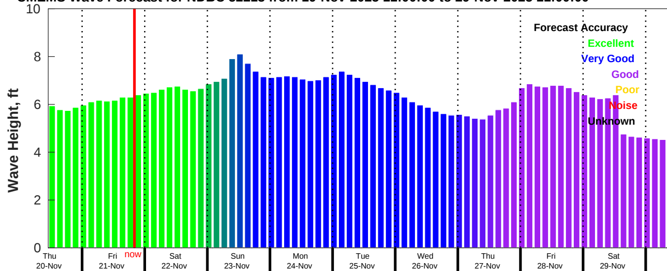
CMEMS Wave Forecast for NDBC 52213 from 19-Nov-2025 11:00:00 to 29-Nov-2025 11:00:00
