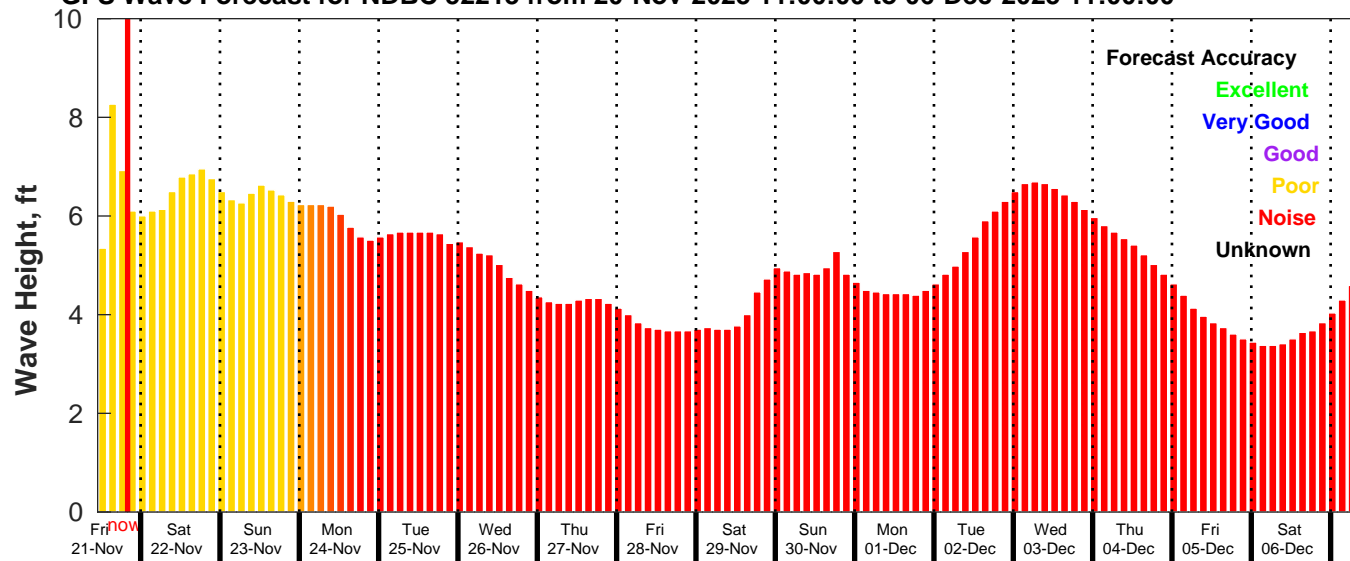
GFS Wave Forecast for NDBC 52213 from 20-Nov-2025 11:00:00 to 06-Dec-2025 11:00:00
