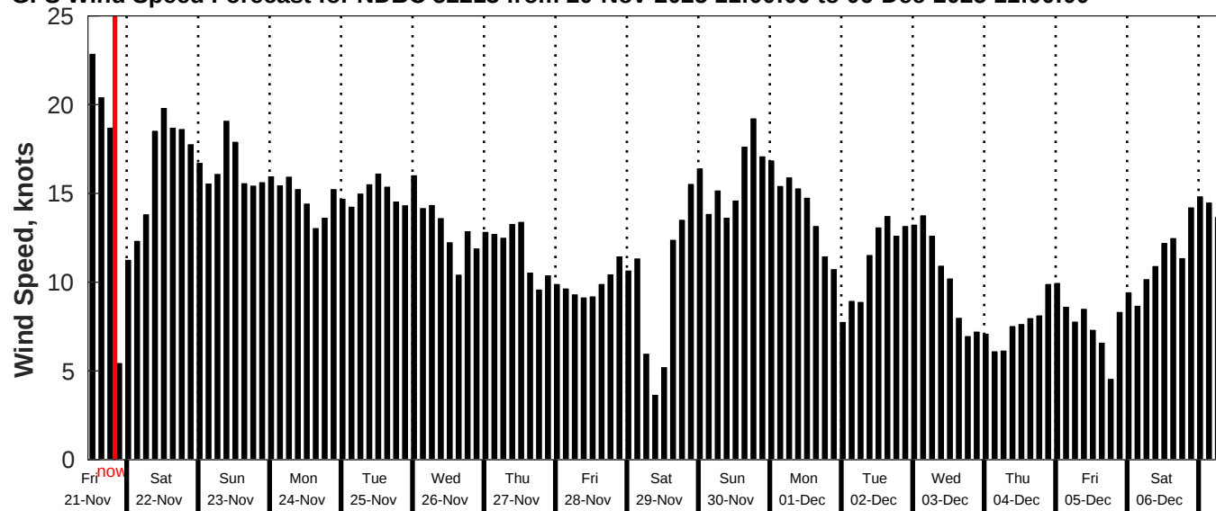
GFS Wind Speed Forecast for NDBC 52213 from 20-Nov-2025 11:00:00 to 06-Dec-2025 11:00:00
