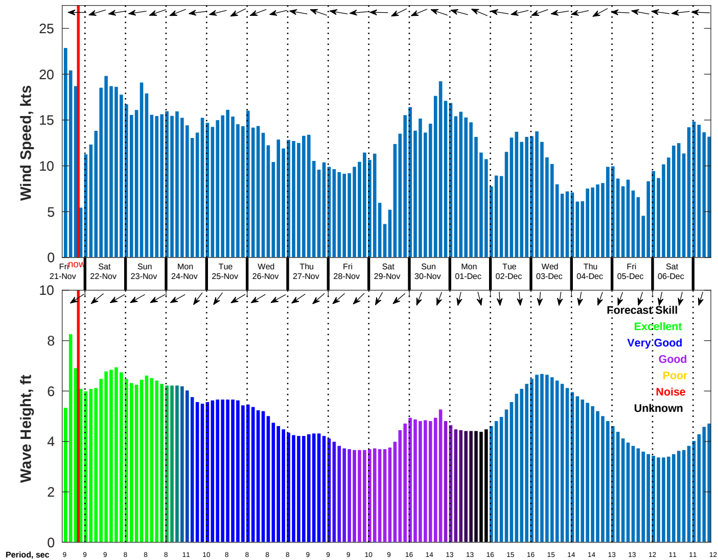
Wind & Wave Forecast for NDBC 52213 from 20-Nov-2025 11:00:00 to 06-Dec-2025 11:00:00
