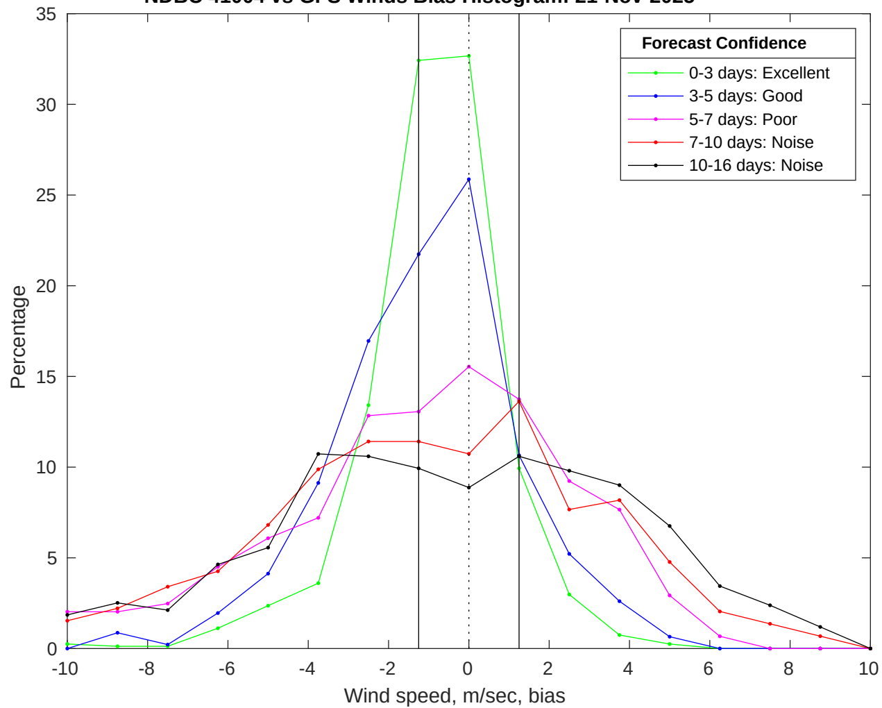
NDBC 41004 vs GFS Winds Bias Histogram: 21-Nov-2025
