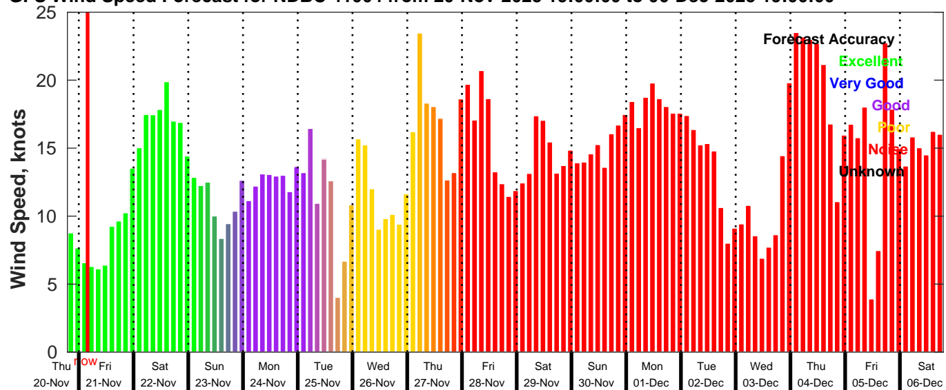
GFS Wind Speed Forecast for NDBC 41004 from 20-Nov-2025 19:00:00 to 06-Dec-2025 19:00:00
