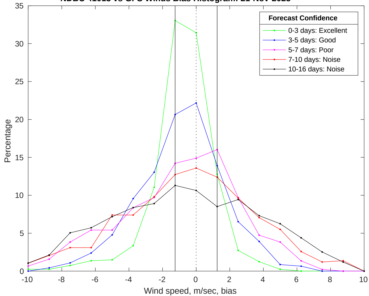
NDBC 41013 vs GFS Winds Bias Histogram: 21-Nov-2025
