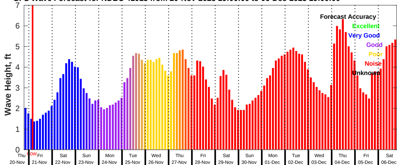
GFS Wave Forecast for NDBC 41013 from 20-Nov-2025 19:00:00 to 06-Dec-2025 19:00:00
