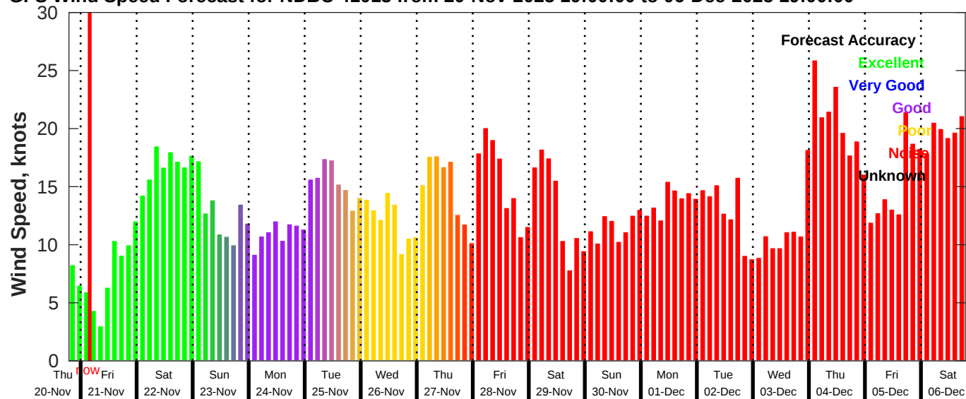
GFS Wind Speed Forecast for NDBC 41013 from 20-Nov-2025 19:00:00 to 06-Dec-2025 19:00:00
