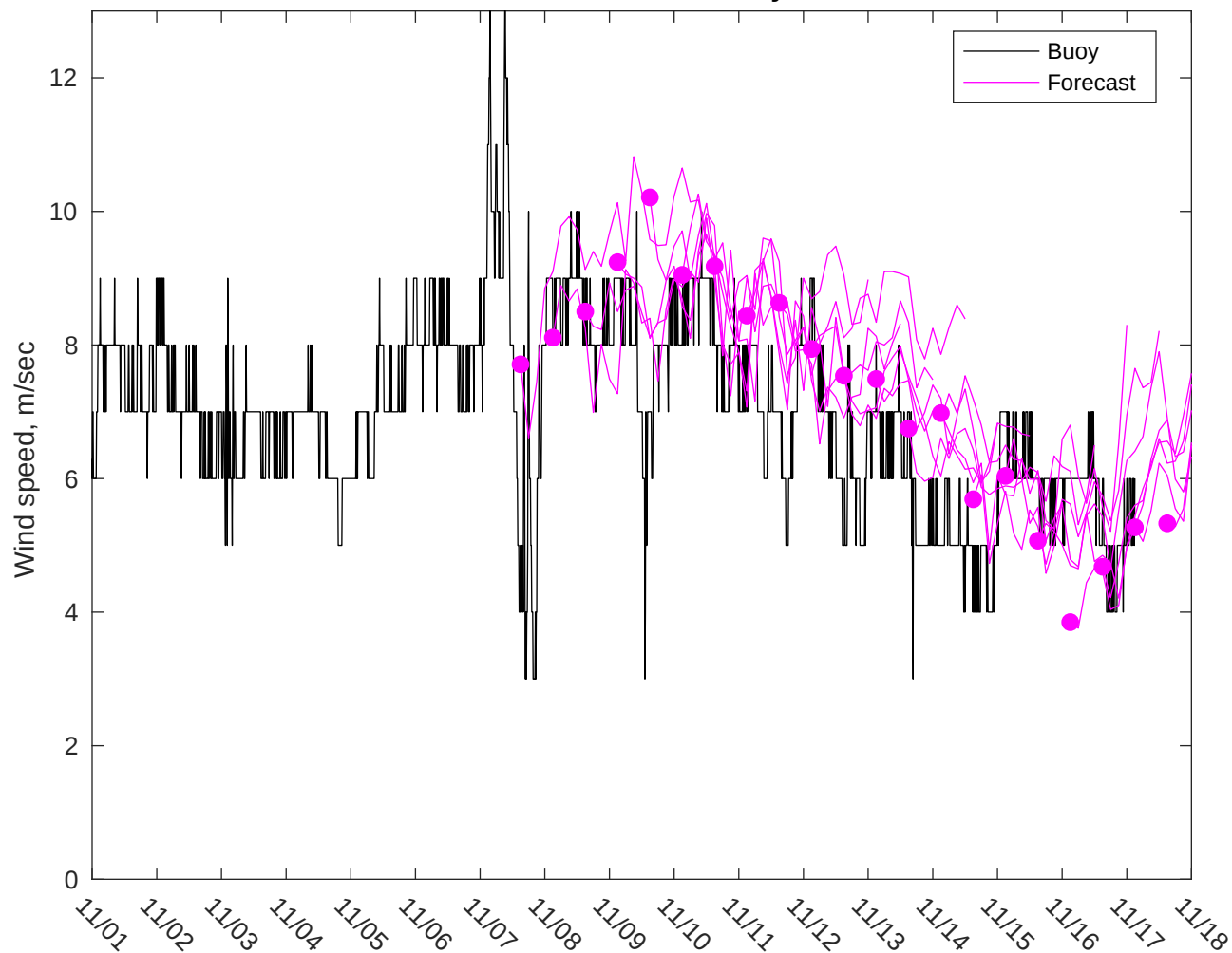
NDBC 41040 vs GFS Winds: 7 to 10 day forecast
