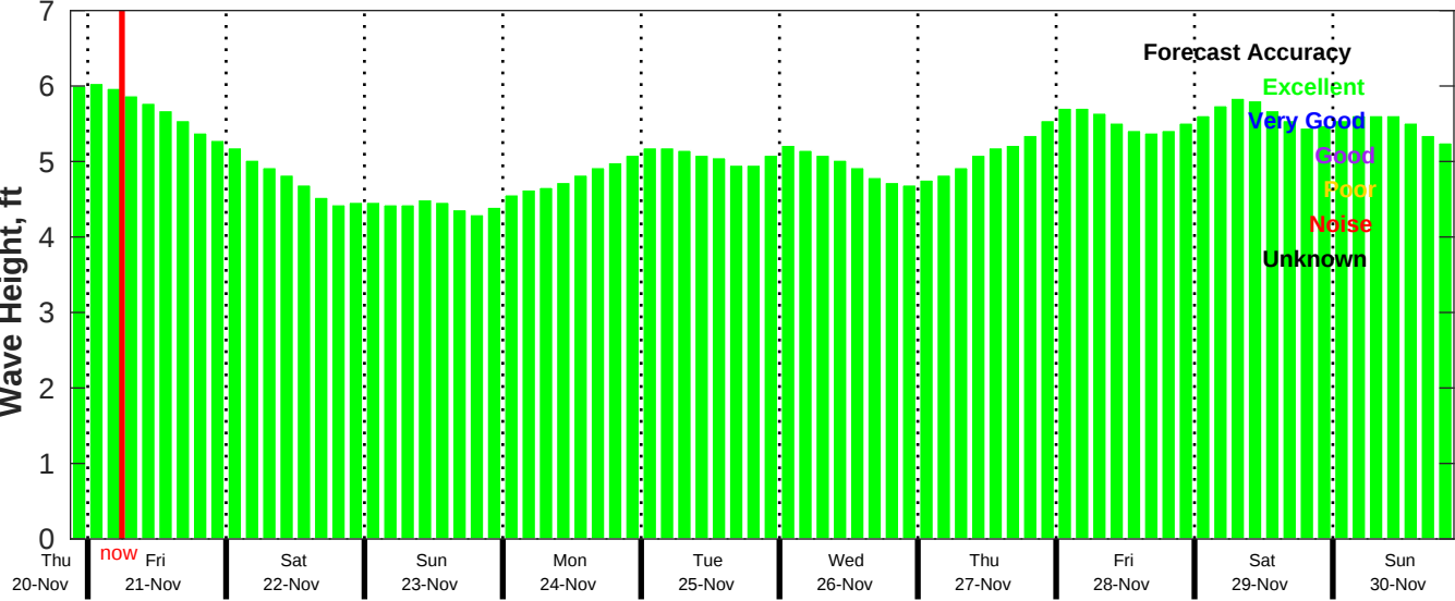
CMEMS Wave Forecast for NDBC 41040 from 20-Nov-2025 21:00:00 to 30-Nov-2025 21:00:00
