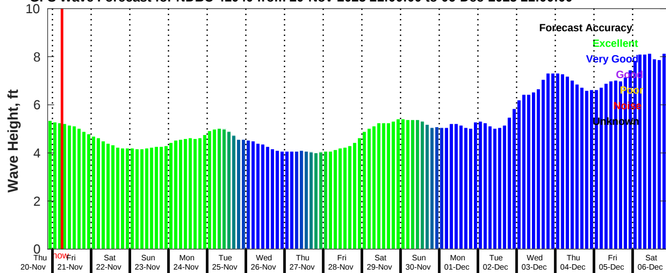
GFS Wave Forecast for NDBC 41040 from 20-Nov-2025 21:00:00 to 06-Dec-2025 21:00:00
