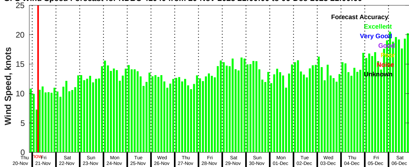
GFS Wind Speed Forecast for NDBC 41040 from 20-Nov-2025 21:00:00 to 06-Dec-2025 21:00:00
