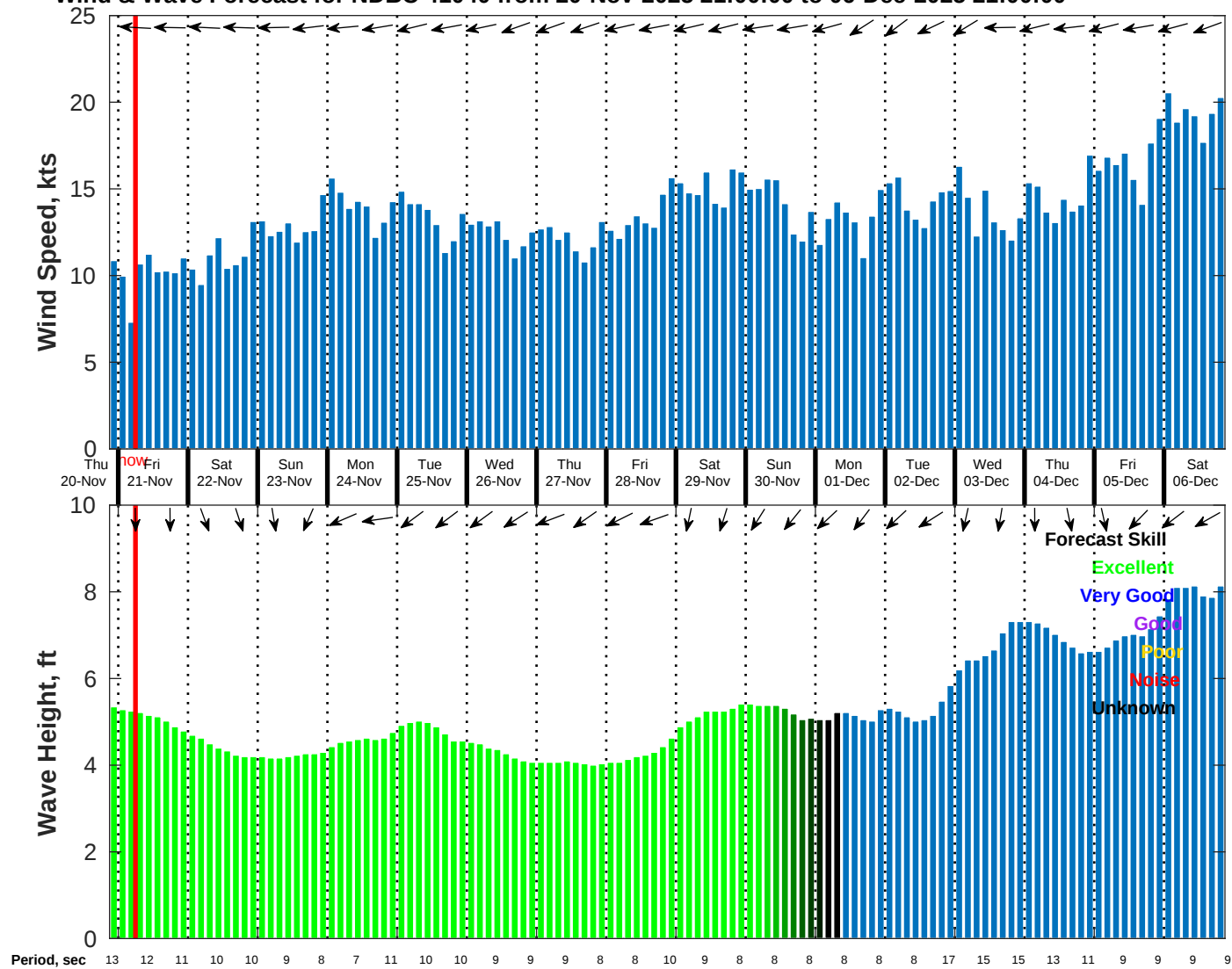
Wind & Wave Forecast for NDBC 41040 from 20-Nov-2025 21:00:00 to 06-Dec-2025 21:00:00
