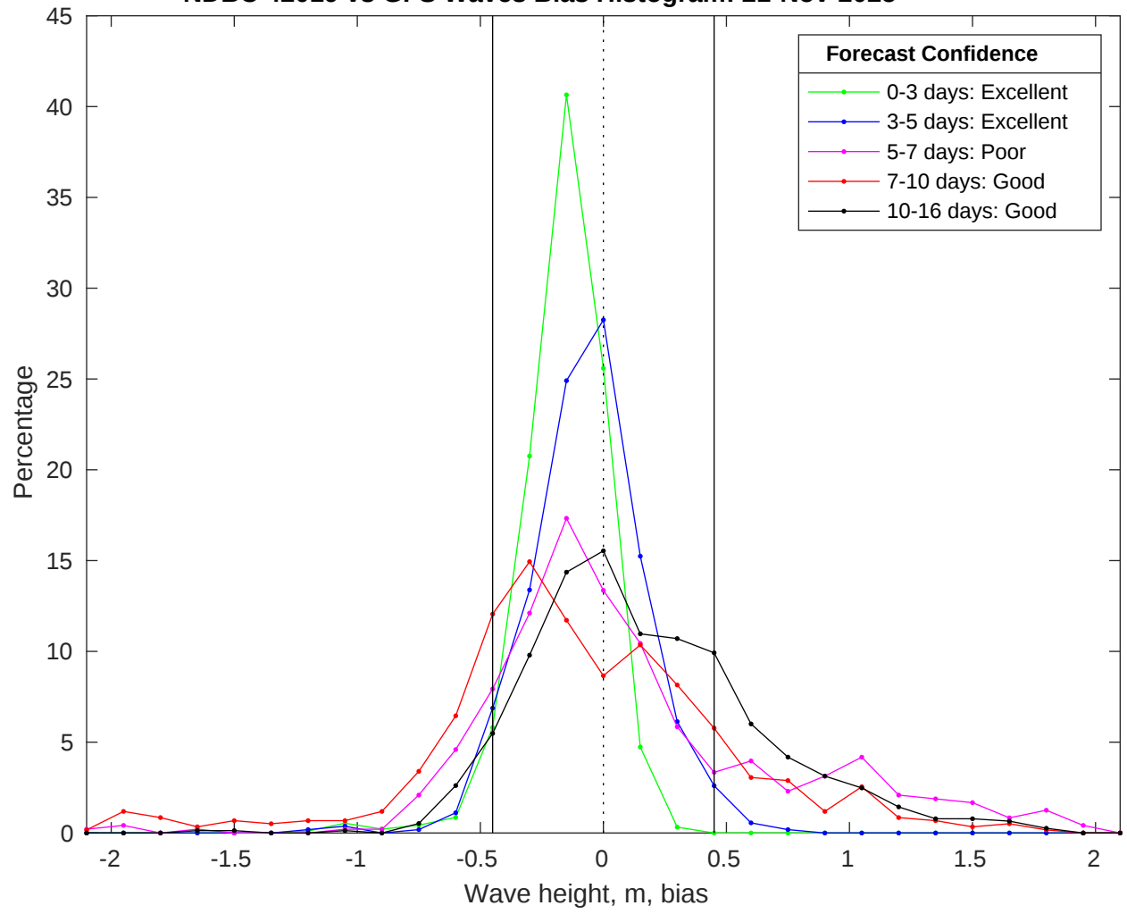
NDBC 42019 vs GFS Waves Bias Histogram: 21-Nov-2025
