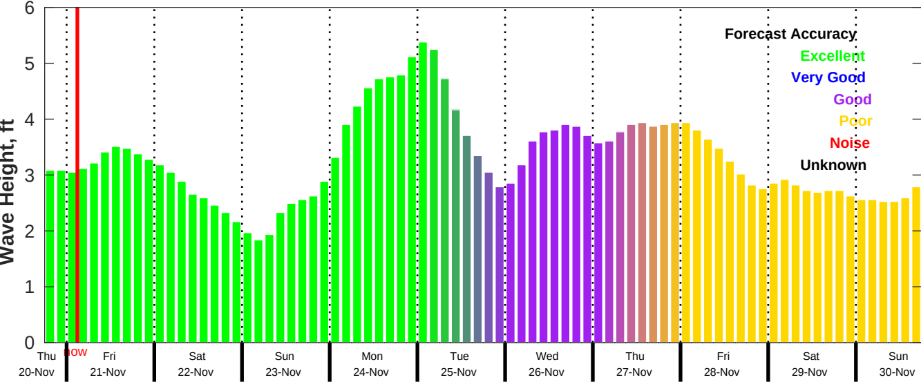
CMEMS Wave Forecast for NDBC 42019 from 20-Nov-2025 18:00:00 to 30-Nov-2025 18:00:00
