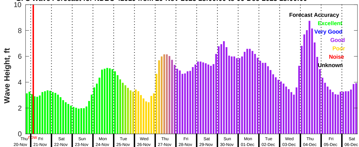
GFS Wave Forecast for NDBC 42019 from 20-Nov-2025 18:00:00 to 06-Dec-2025 18:00:00
