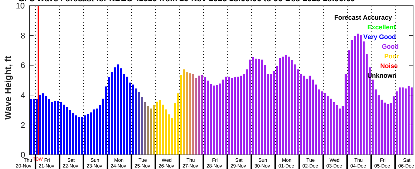
GFS Wave Forecast for NDBC 42020 from 20-Nov-2025 18:00:00 to 06-Dec-2025 18:00:00
