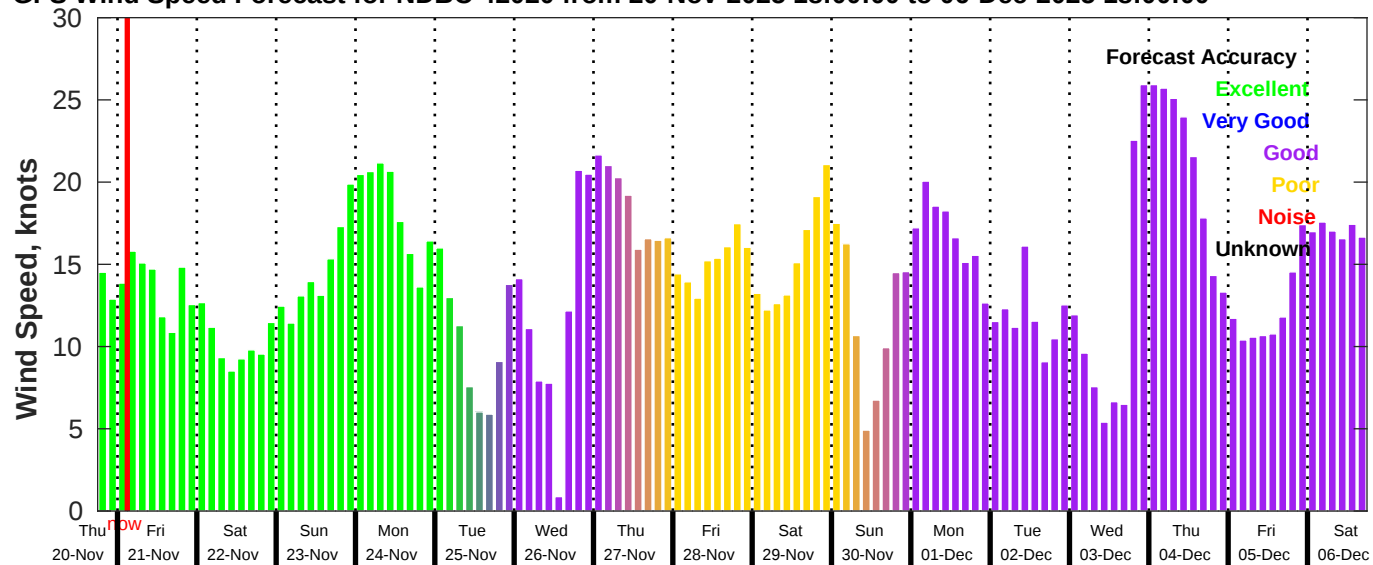
GFS Wind Speed Forecast for NDBC 42020 from 20-Nov-2025 18:00:00 to 06-Dec-2025 18:00:00
