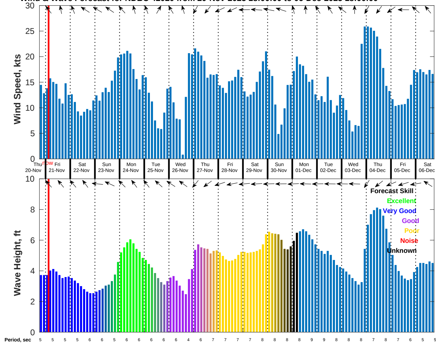
Wind & Wave Forecast for NDBC 42020 from 20-Nov-2025 18:00:00 to 06-Dec-2025 18:00:00
