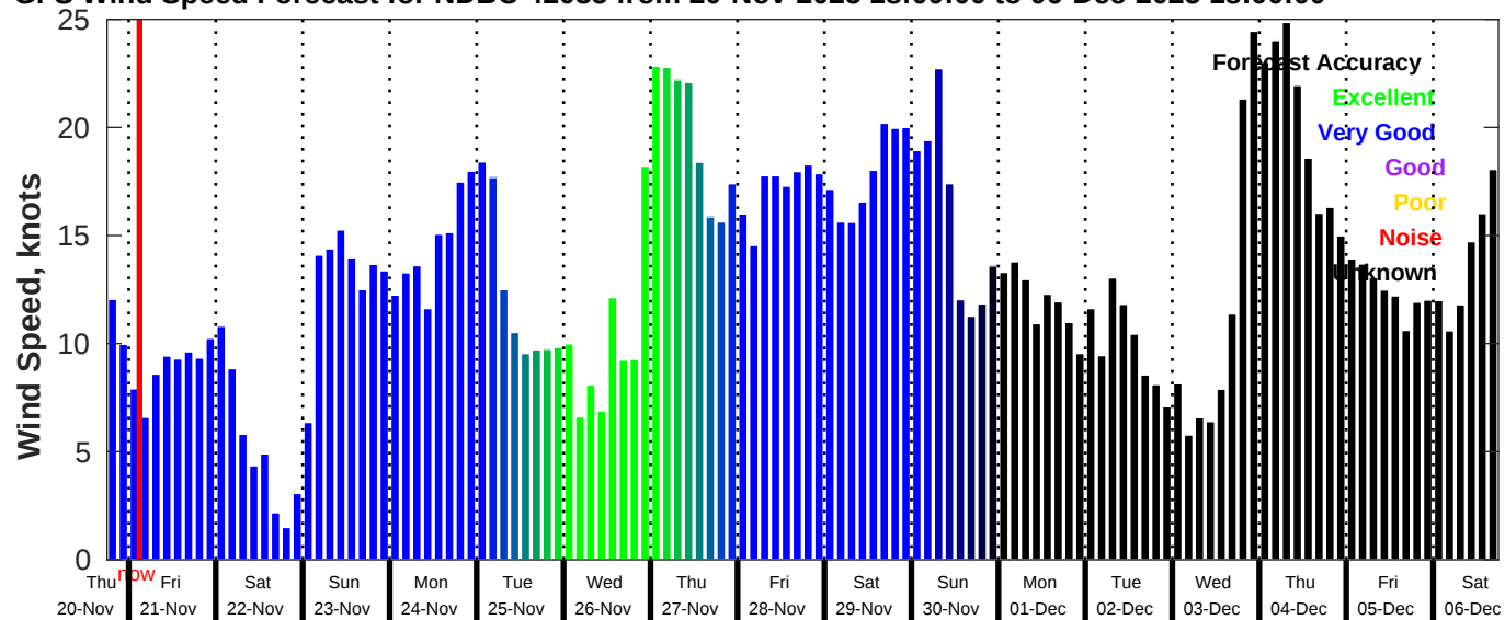
GFS Wind Speed Forecast for NDBC 42035 from 20-Nov-2025 18:00:00 to 06-Dec-2025 18:00:00
