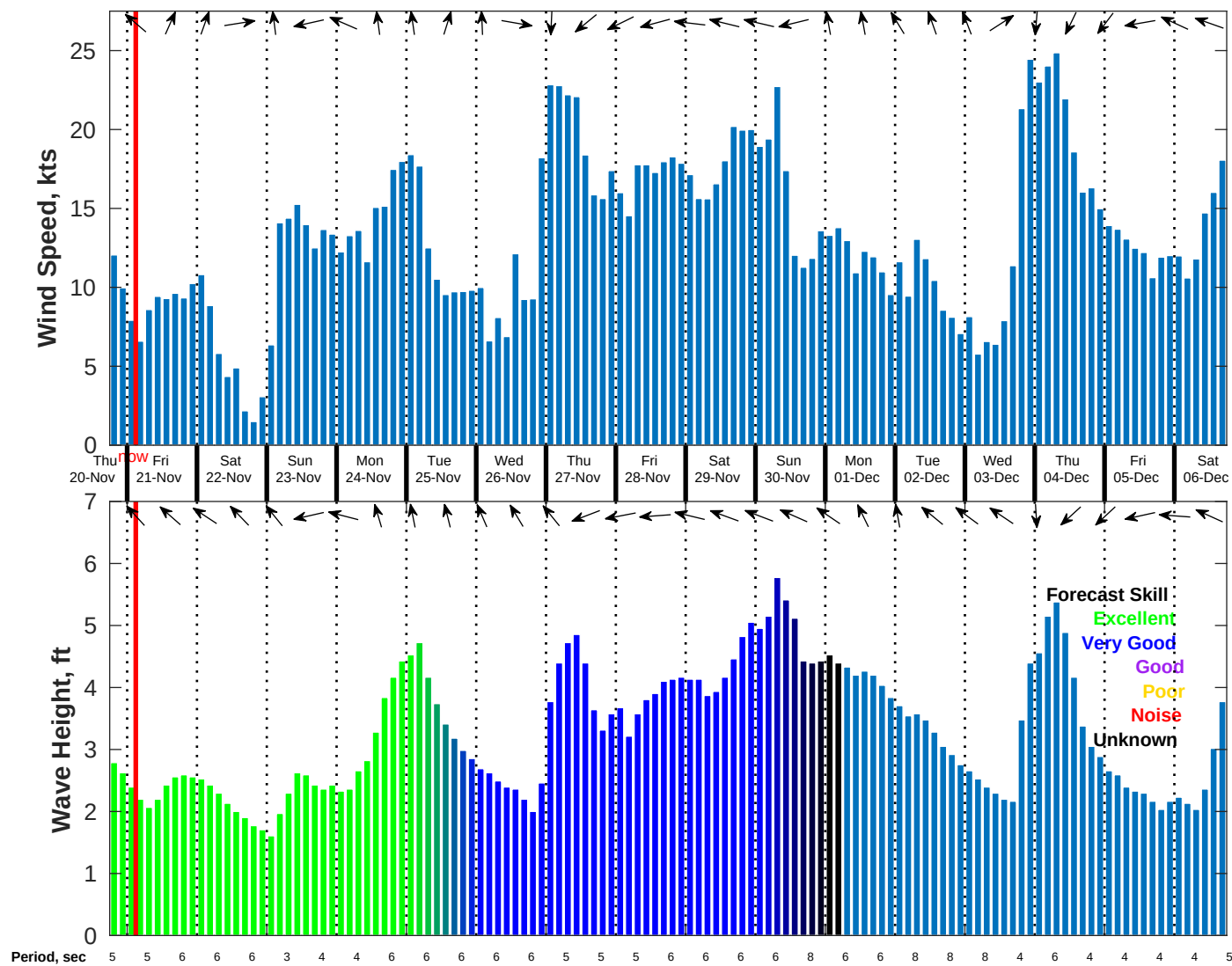
Wind & Wave Forecast for NDBC 42035 from 20-Nov-2025 18:00:00 to 06-Dec-2025 18:00:00
