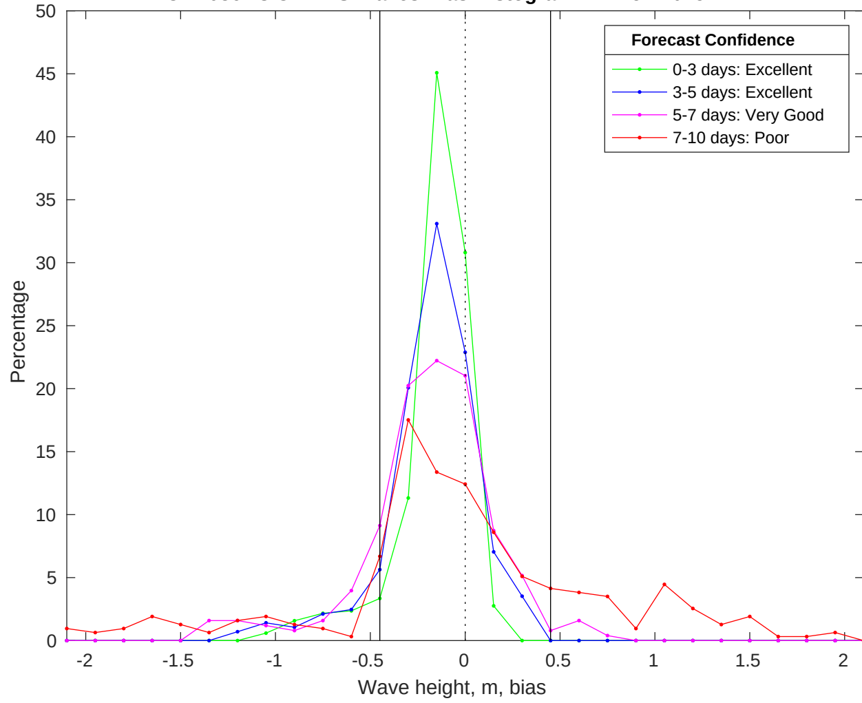
NDBC 42036 vs CMEMS Waves Bias Histogram: 21-Nov-2025
