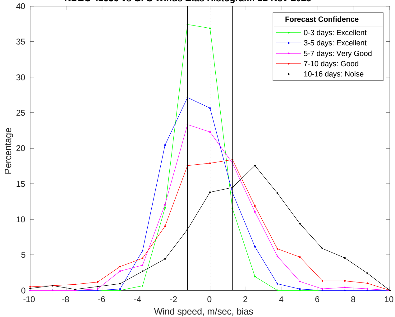
NDBC 42036 vs GFS Winds Bias Histogram: 21-Nov-2025
