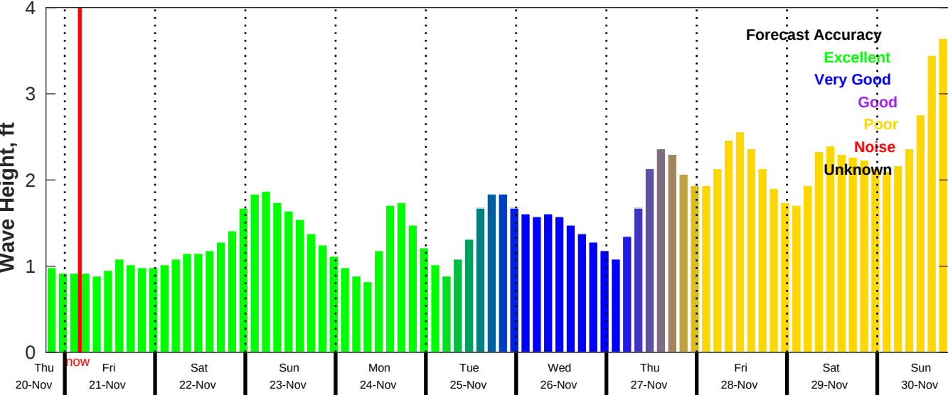
CMEMS Wave Forecast for NDBC 42036 from 20-Nov-2025 19:00:00 to 30-Nov-2025 19:00:00
