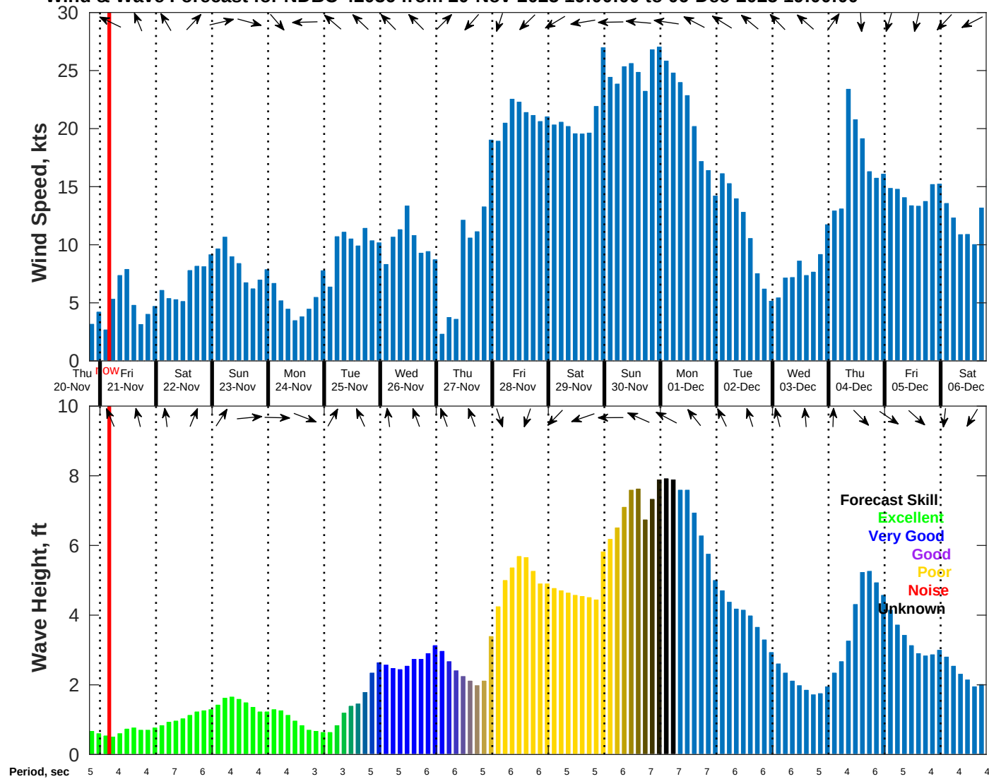
Wind & Wave Forecast for NDBC 42036 from 20-Nov-2025 19:00:00 to 06-Dec-2025 19:00:00
