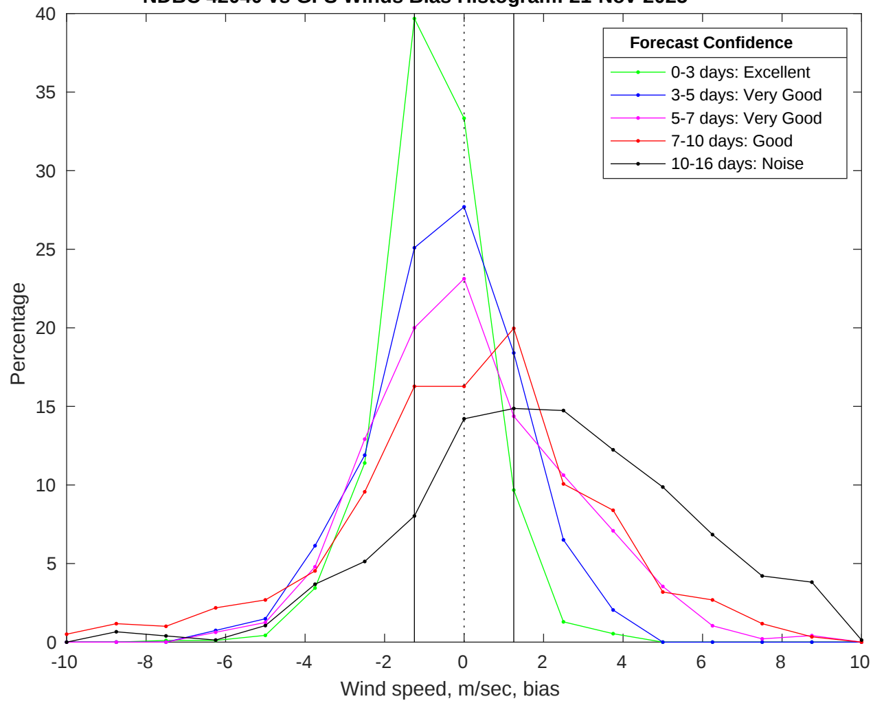
NDBC 42040 vs GFS Winds Bias Histogram: 21-Nov-2025
