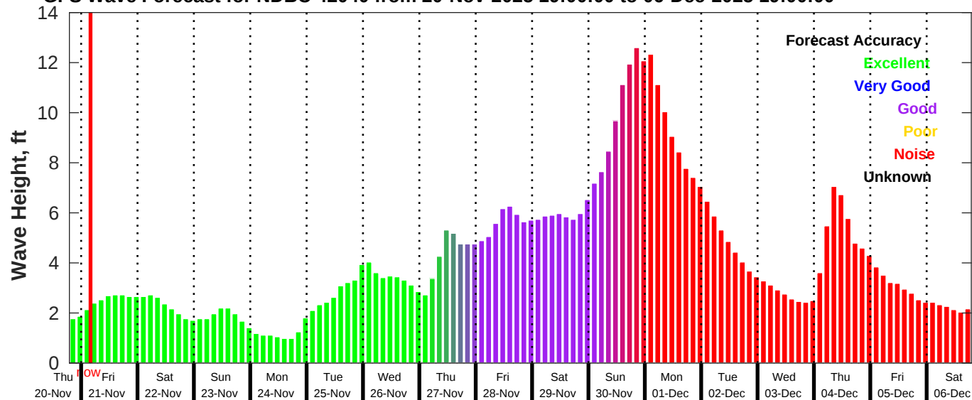
GFS Wave Forecast for NDBC 42040 from 20-Nov-2025 19:00:00 to 06-Dec-2025 19:00:00
