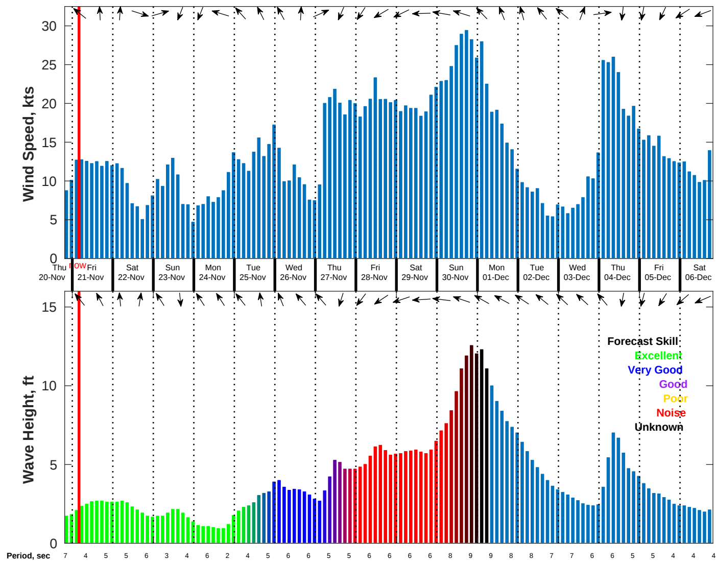
Wind & Wave Forecast for NDBC 42040 from 20-Nov-2025 19:00:00 to 06-Dec-2025 19:00:00
