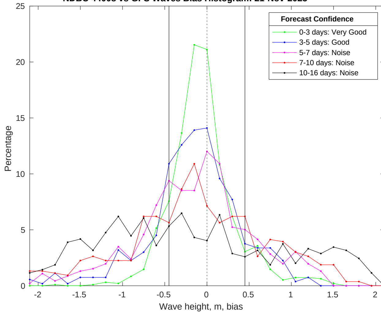
NDBC 44008 vs GFS Waves Bias Histogram: 21-Nov-2025
