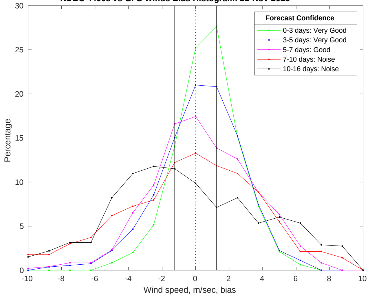
NDBC 44008 vs GFS Winds Bias Histogram: 21-Nov-2025
