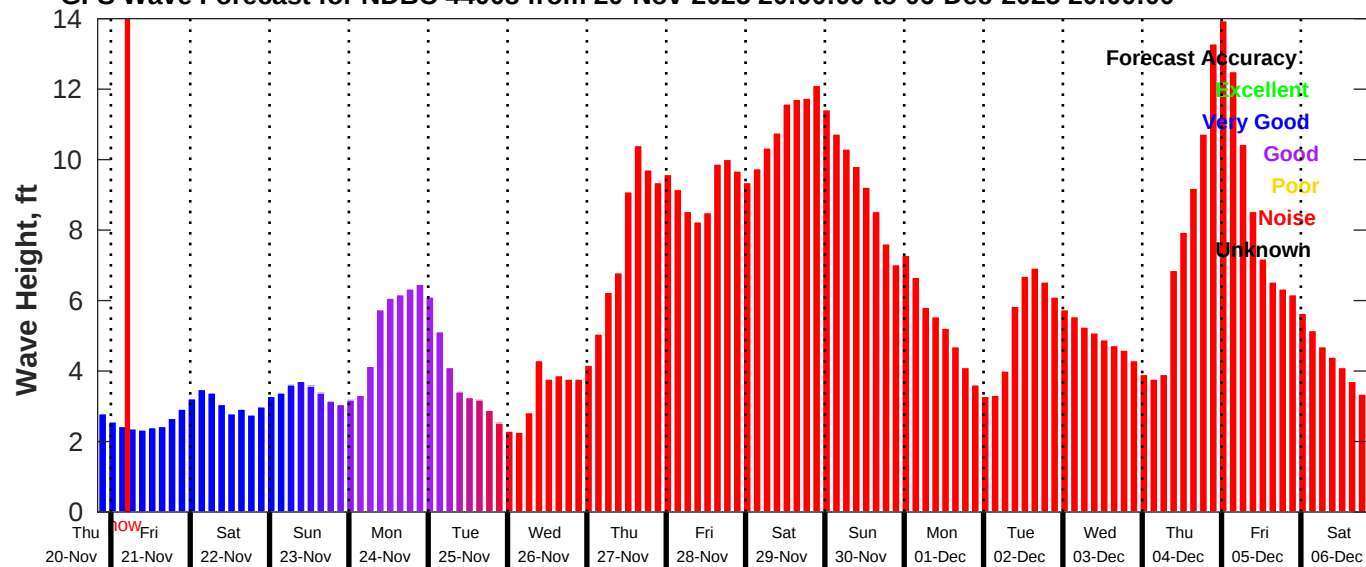
GFS Wave Forecast for NDBC 44008 from 20-Nov-2025 20:00:00 to 06-Dec-2025 20:00:00
