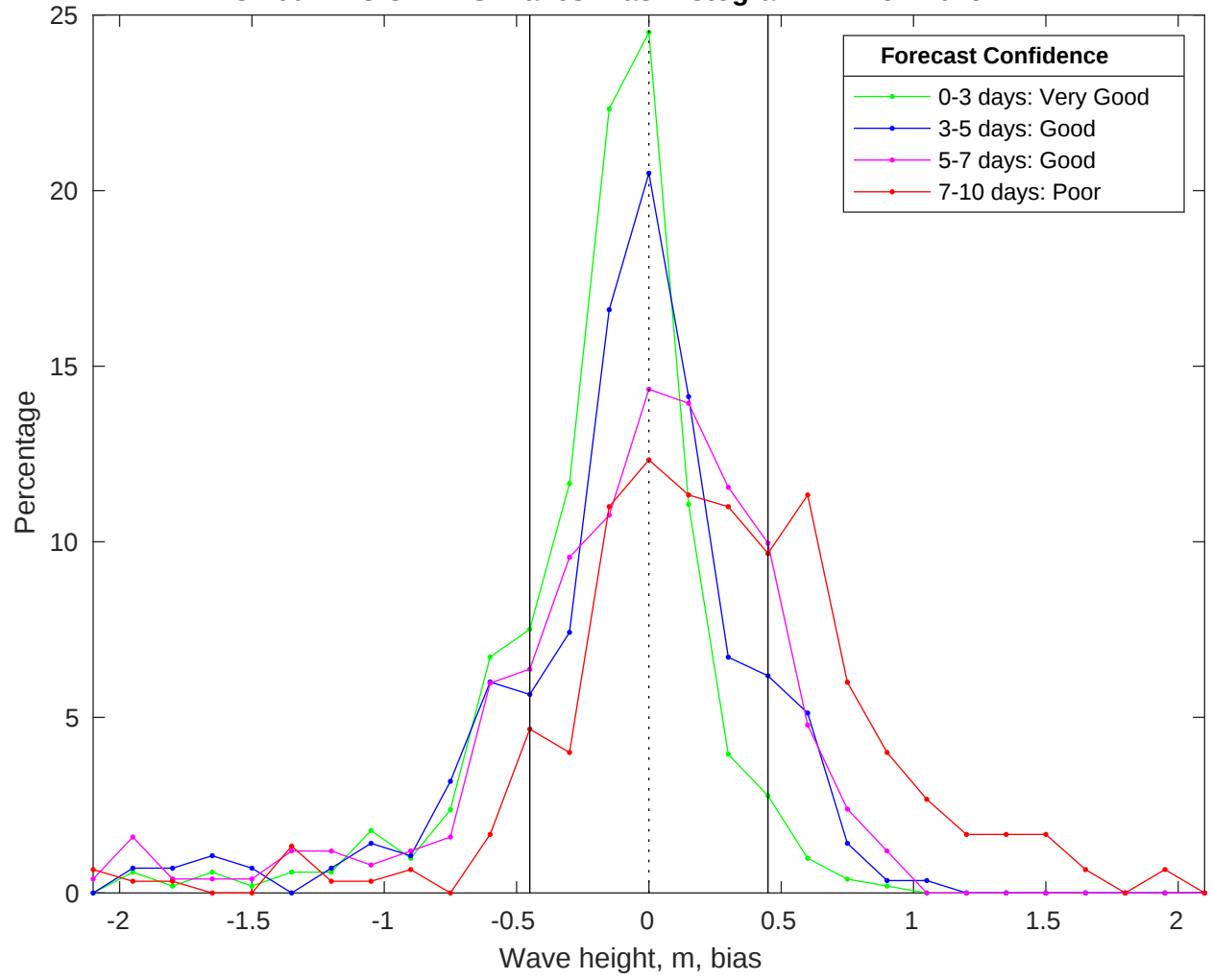
NDBC 46011 vs CMEMS Waves Bias Histogram: 21-Nov-2025
