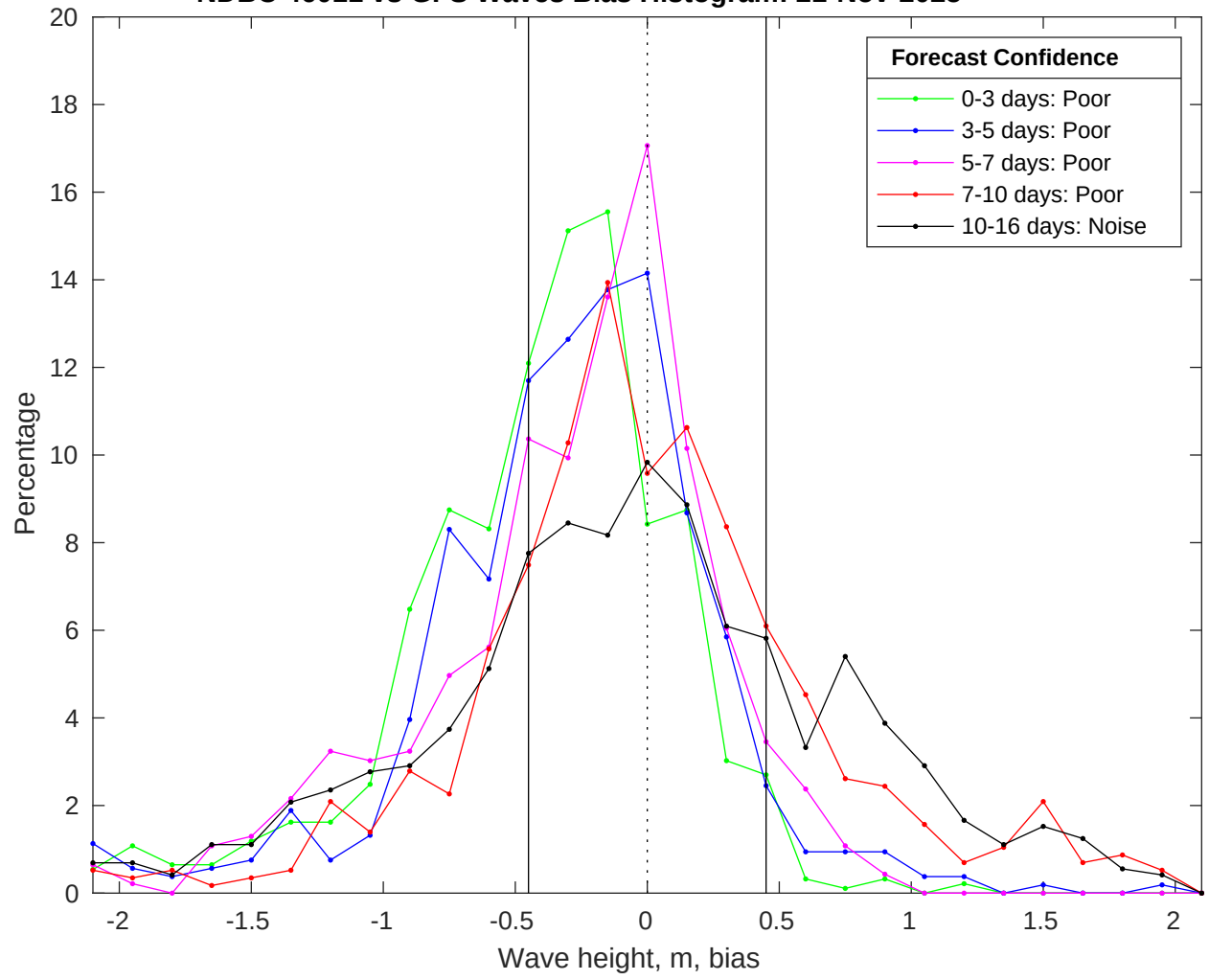
NDBC 46011 vs GFS Waves Bias Histogram: 21-Nov-2025
