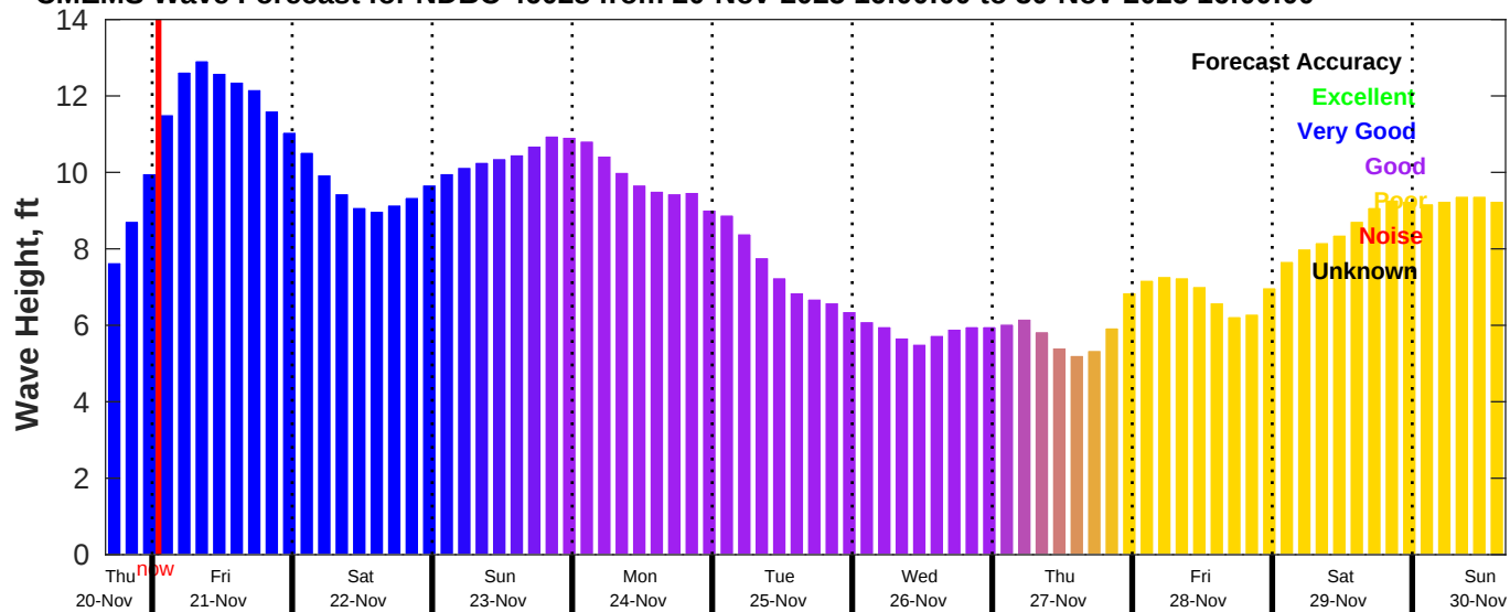
CMEMS Wave Forecast for NDBC 46028 from 20-Nov-2025 16:00:00 to 30-Nov-2025 16:00:00
