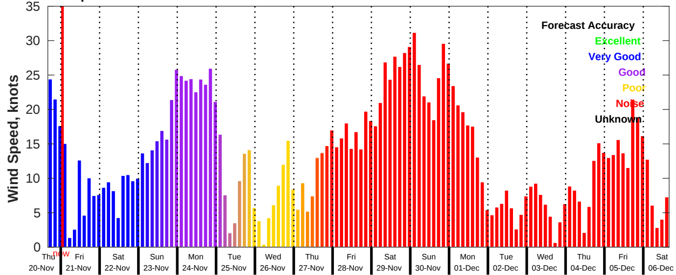
GFS Wind Speed Forecast for NDBC 46028 from 20-Nov-2025 16:00:00 to 06-Dec-2025 16:00:00
