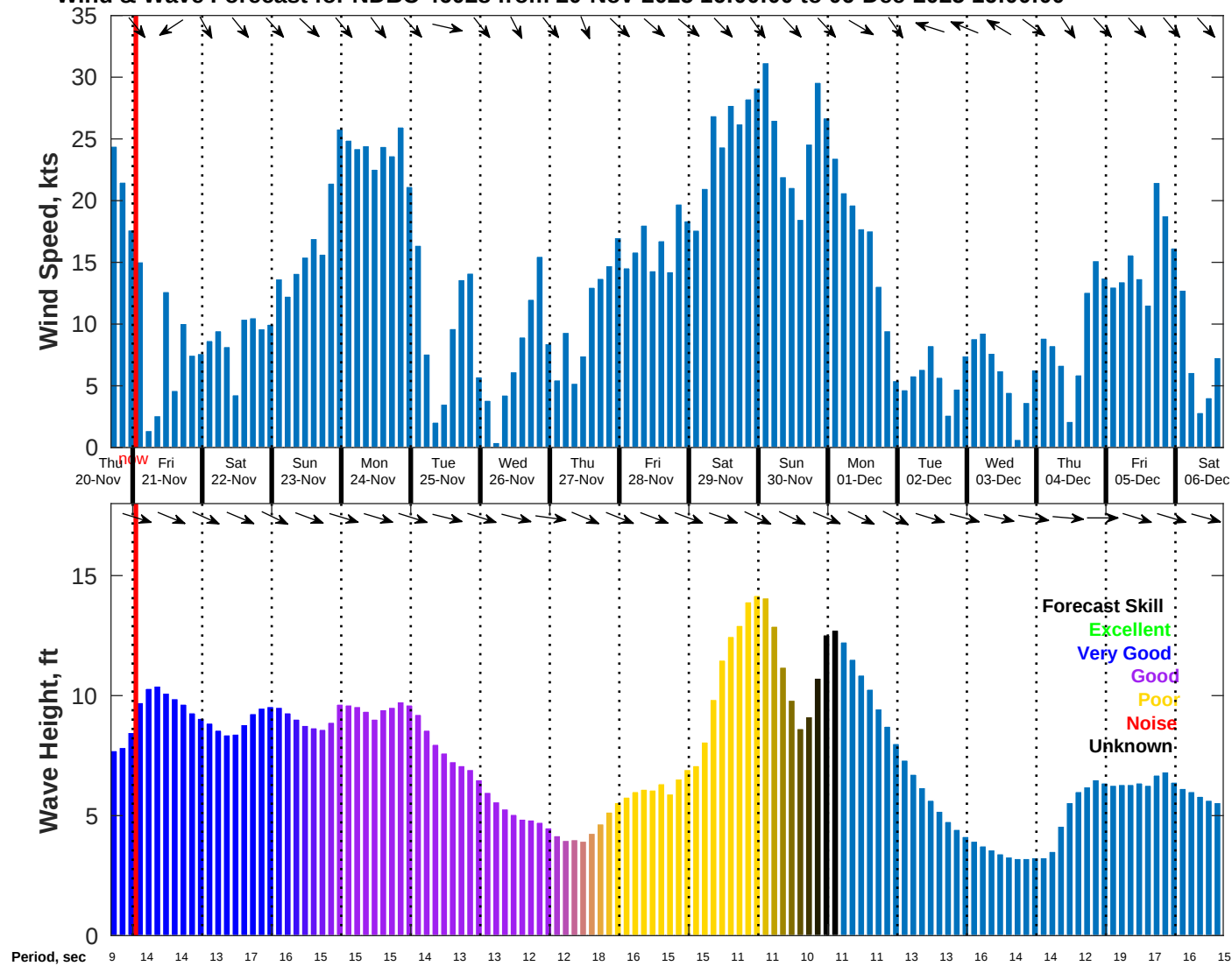
Wind & Wave Forecast for NDBC 46028 from 20-Nov-2025 16:00:00 to 06-Dec-2025 16:00:00
