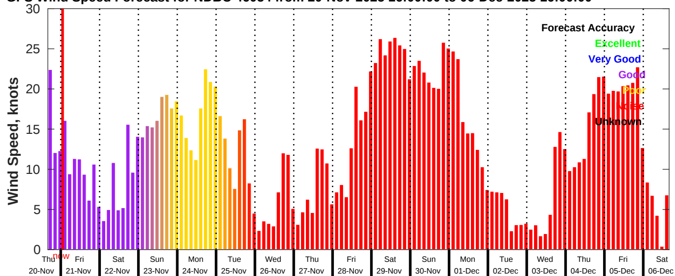
GFS Wind Speed Forecast for NDBC 46054 from 20-Nov-2025 16:00:00 to 06-Dec-2025 16:00:00
