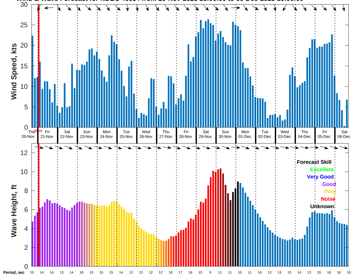
Wind & Wave Forecast for NDBC 46054 from 20-Nov-2025 16:00:00 to 06-Dec-2025 16:00:00
