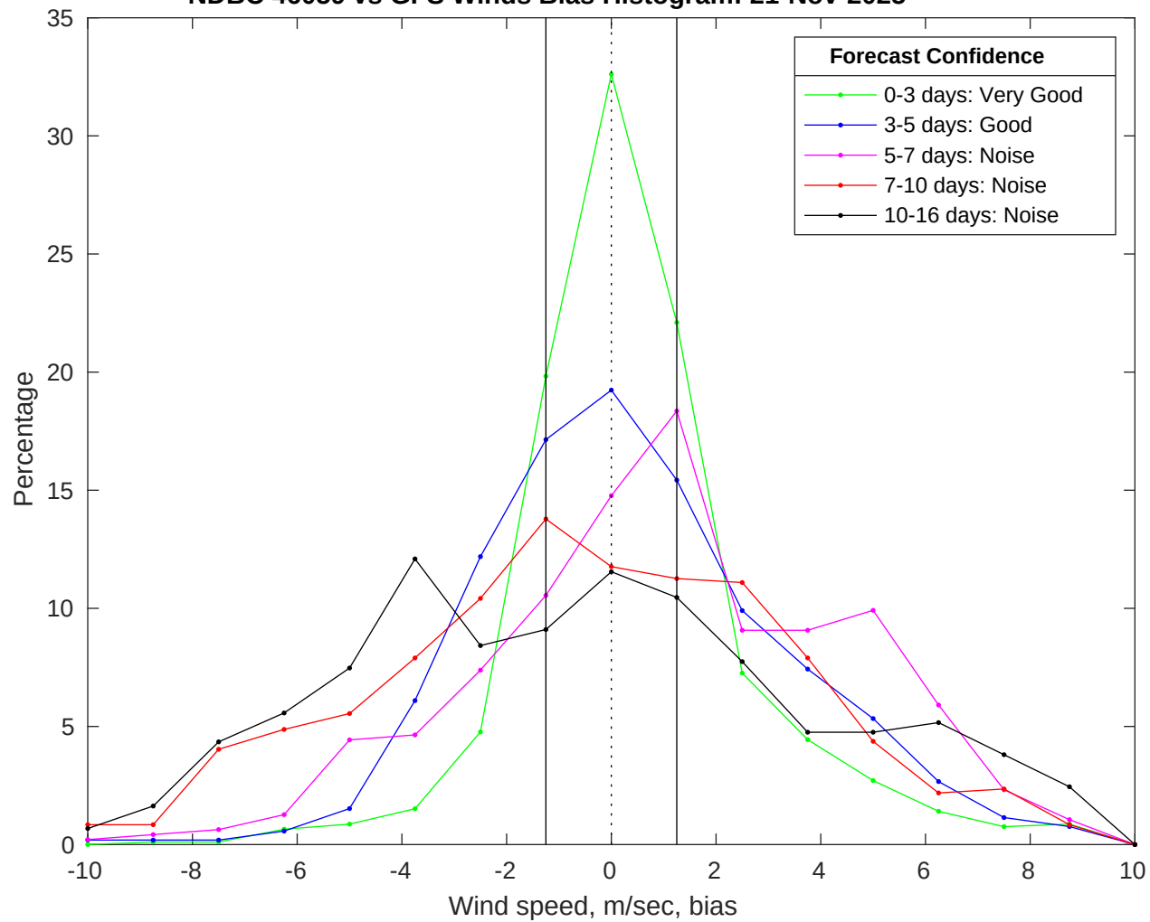
NDBC 46059 vs GFS Winds Bias Histogram: 21-Nov-2025
