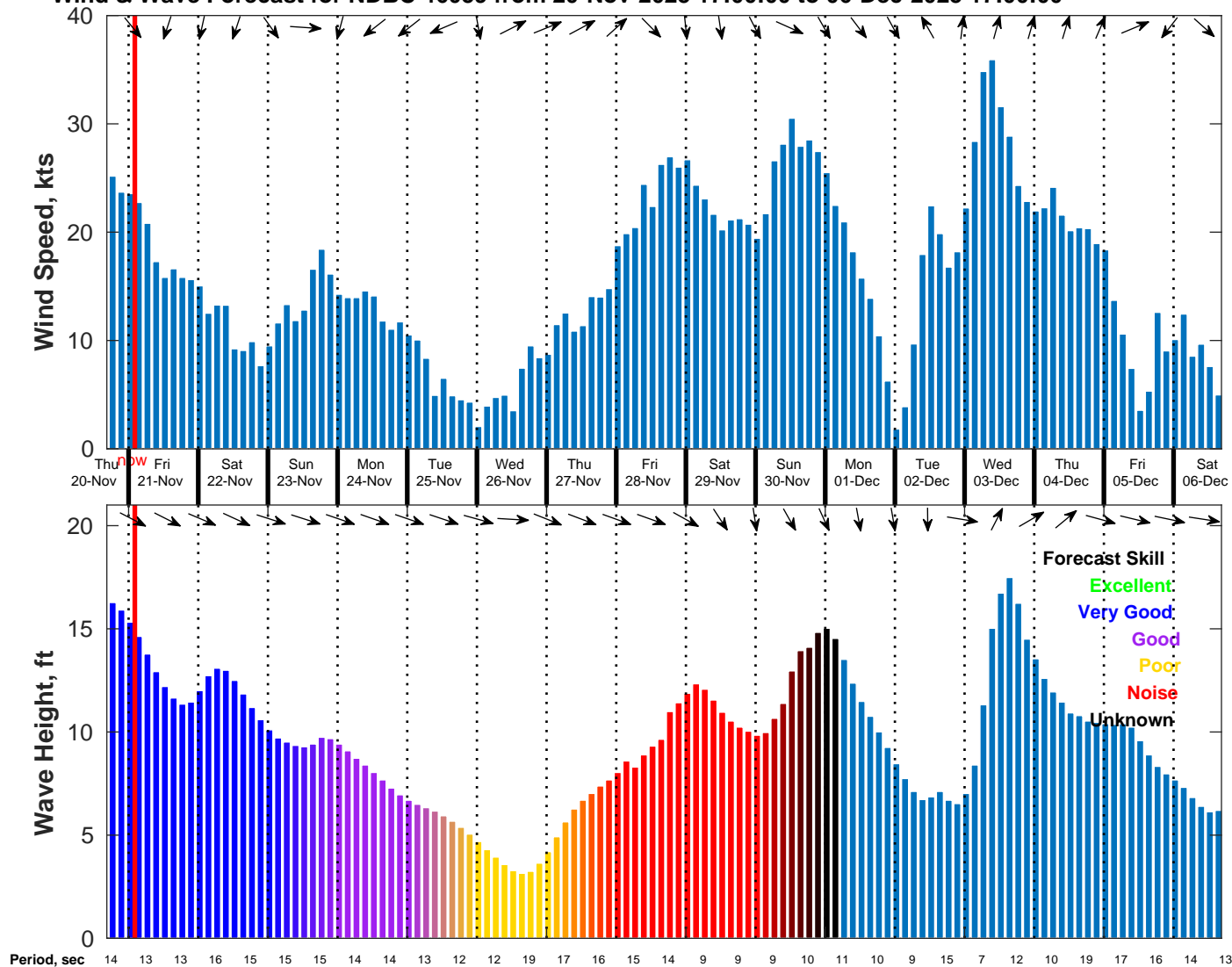
Wind & Wave Forecast for NDBC 46059 from 20-Nov-2025 17:00:00 to 06-Dec-2025 17:00:00
