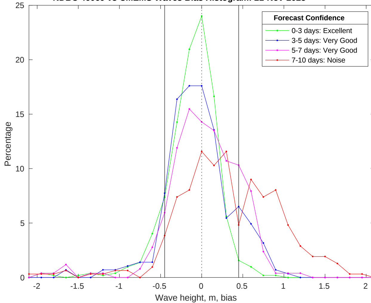
NDBC 46069 vs CMEMS Waves Bias Histogram: 21-Nov-2025
