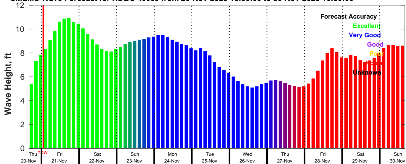
CMEMS Wave Forecast for NDBC 46069 from 20-Nov-2025 16:00:00 to 30-Nov-2025 16:00:00
