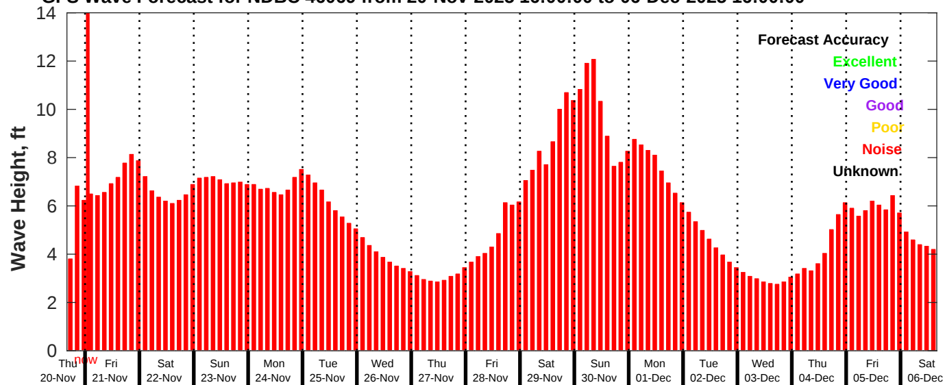
GFS Wave Forecast for NDBC 46069 from 20-Nov-2025 16:00:00 to 06-Dec-2025 16:00:00
